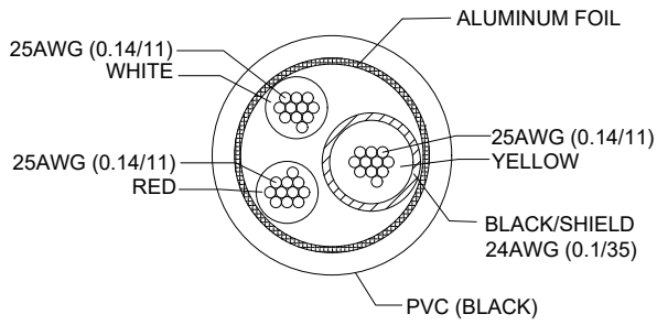
CABLE BUILDUP
