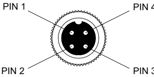
4 PIN FEMALE MATING FACE
