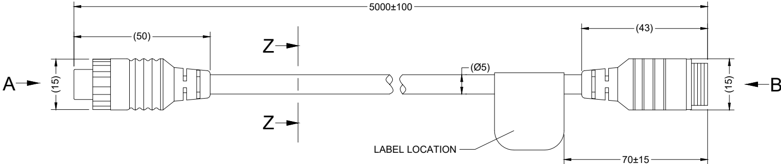
VIEW A
